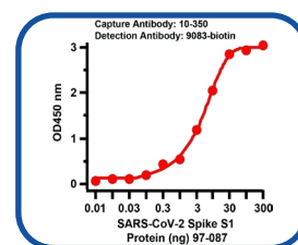
SARS-CoV-2 (COVID-19) Nucleocapsid Matched Pair Cat. No. MPS-0002 Capture Cat. No. 10-350 (2ug/ml) Detection Cat. No. 9083-biotin (1ug/ml)
