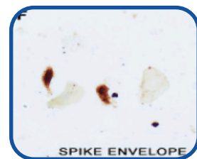
SARS-CoV-2 Envelope Antibody Cat. No. 3531 IHC analysis of envelope protein in COVID-19 patient lung. (Nuovo et al., 2020)
